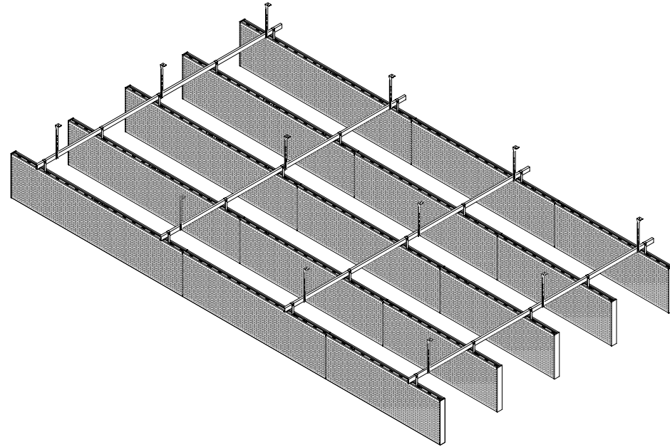
BAFFLE MODULES ISO VIEW CONTINUOUS RUNS GRID HANGING
